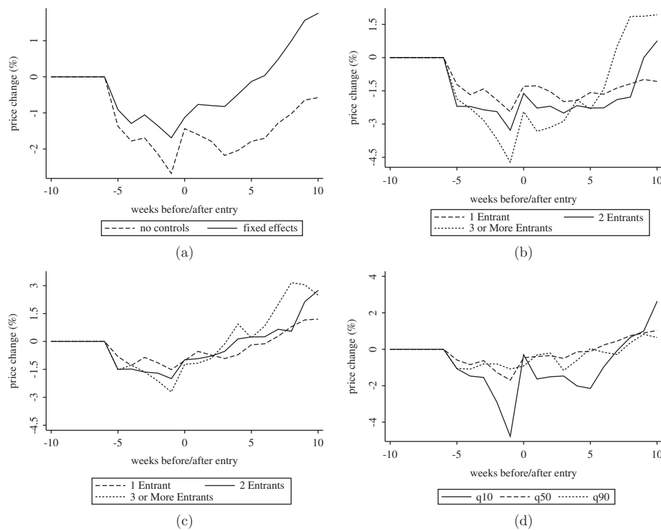
Figure 1. Effect on incumbent prices before and after entry. (a) OLS regression, (b) subsample regression (no controls), (c) subsample regression (incl. controls), (d) quantile regression.
